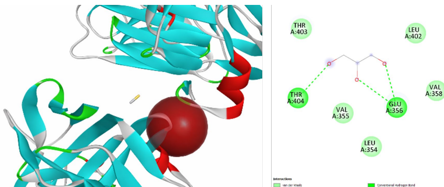
Figure 3. Docking of Sulphanoids with the Targeted Site
