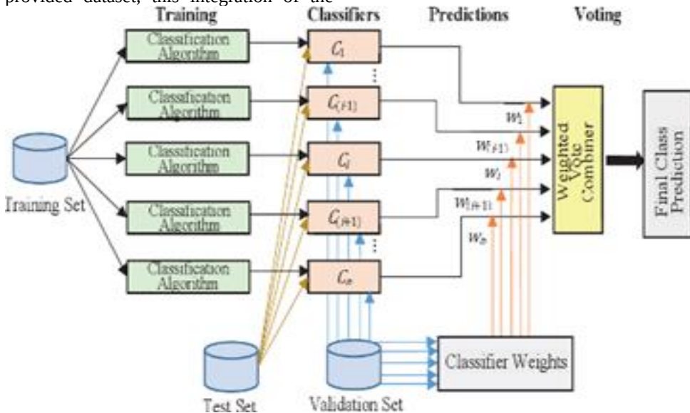
FIGURE 6. Voting ensemble classifier (CNN, LSTM, DNN)
