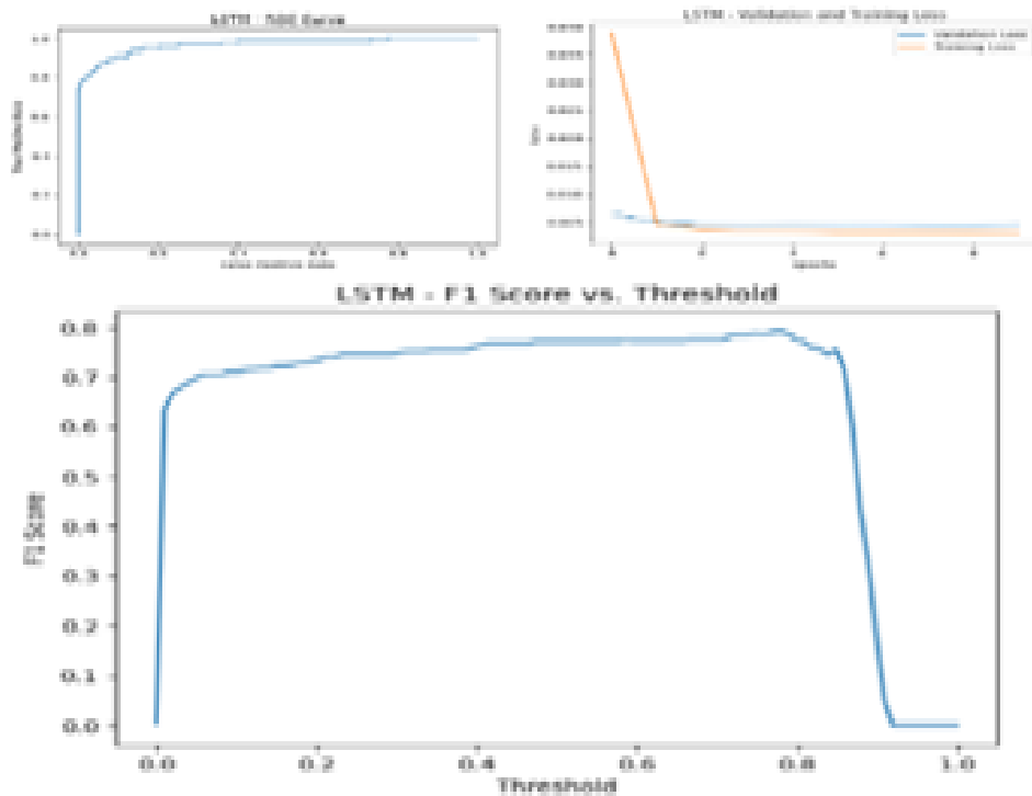
FIGURE 14. Dense neural network (ROC, validation & training, F1)
