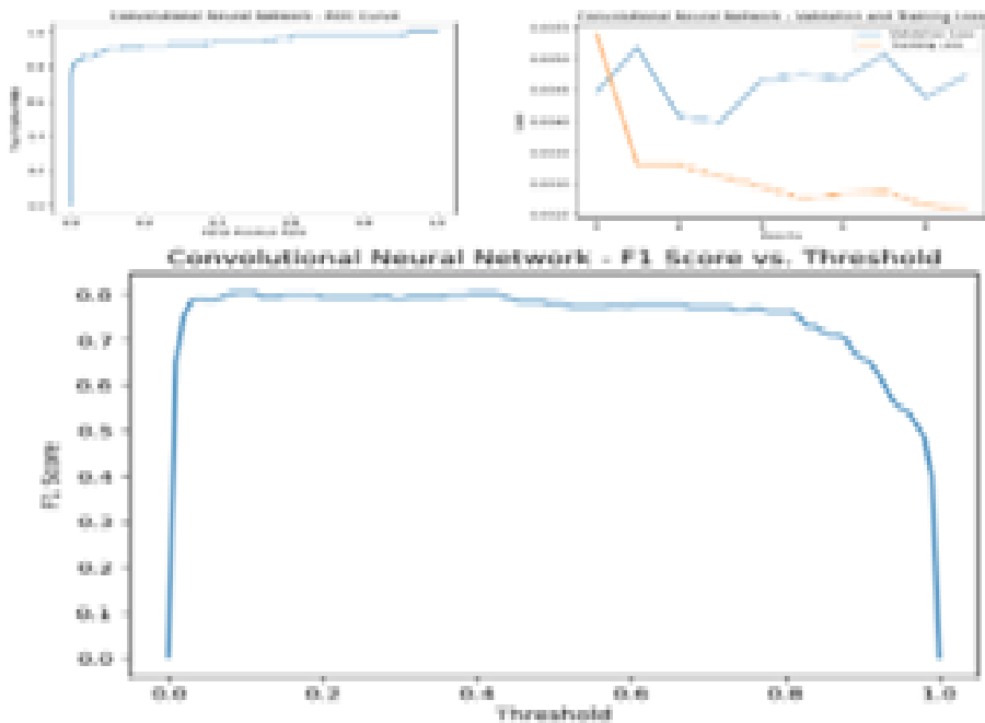
FIGURE 12. CNN (ROC, validation & training)
