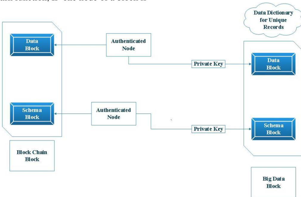
Fig. 3. Integrated new proposed model
