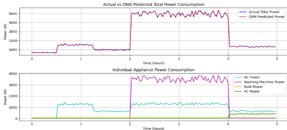
FIGURE 10. DNN predictions based on total power
